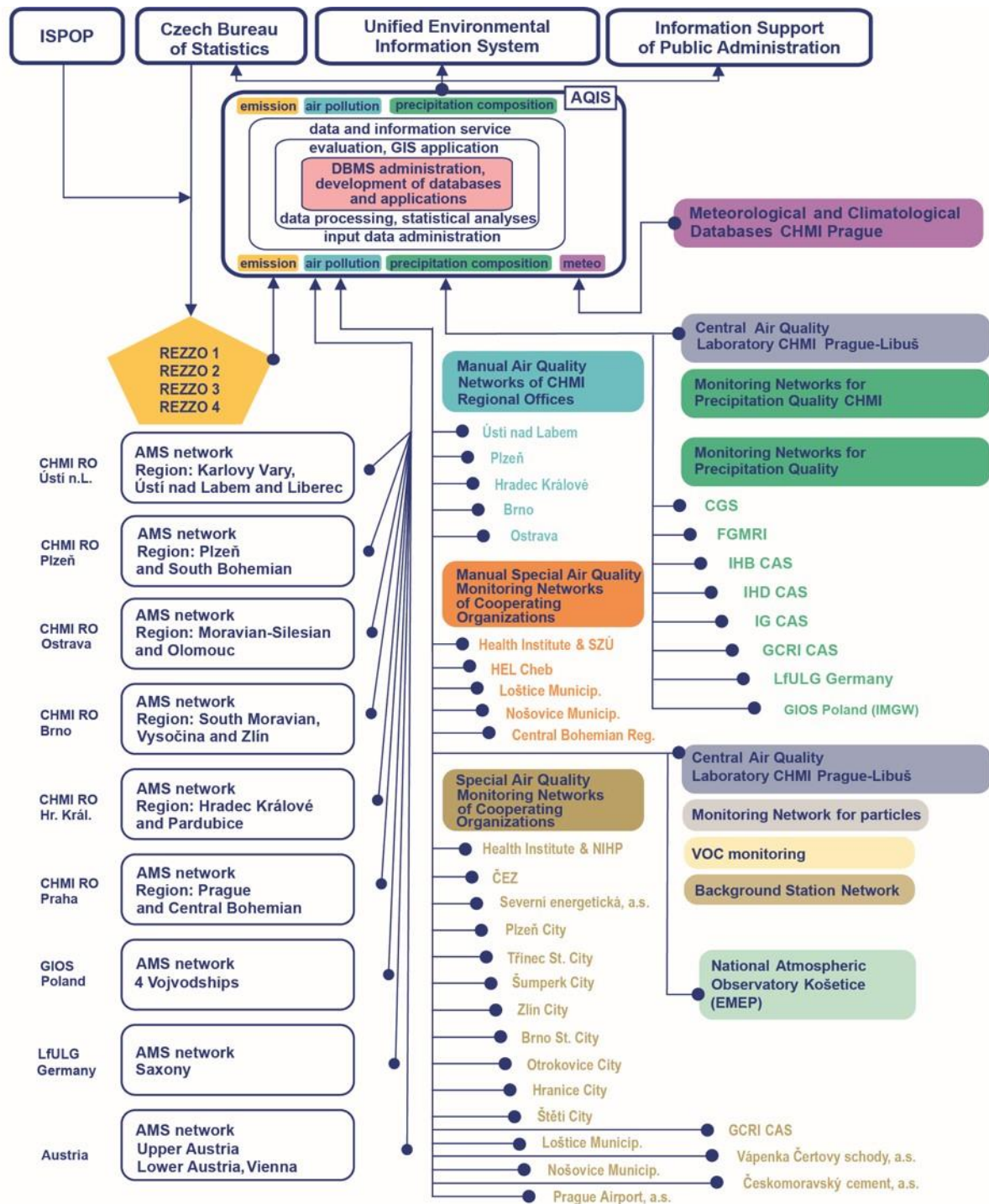
Fig. 1 Scheme of the AQIS links to data sources and cooperating systems in 2019
