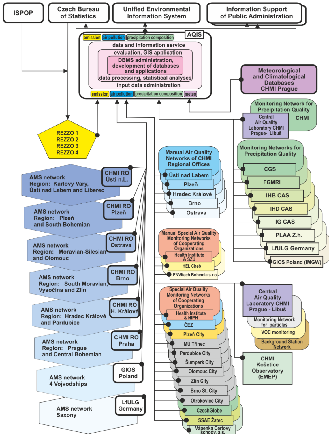
Fig. 1 Scheme of the AQIS links to data sources and cooperating systems in 2015
