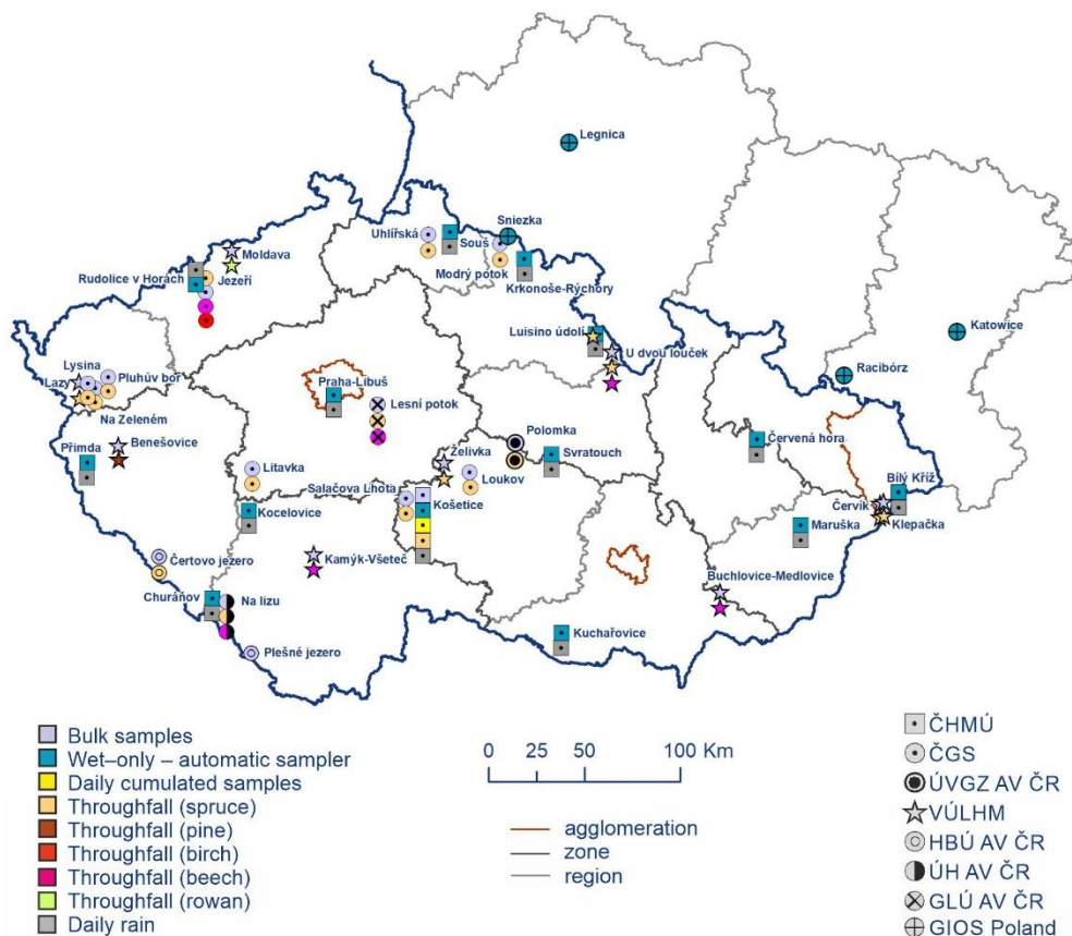
Fig. 13 Station networks monitoring atmospheric precipitation quality and atmospheric deposition, 2020
