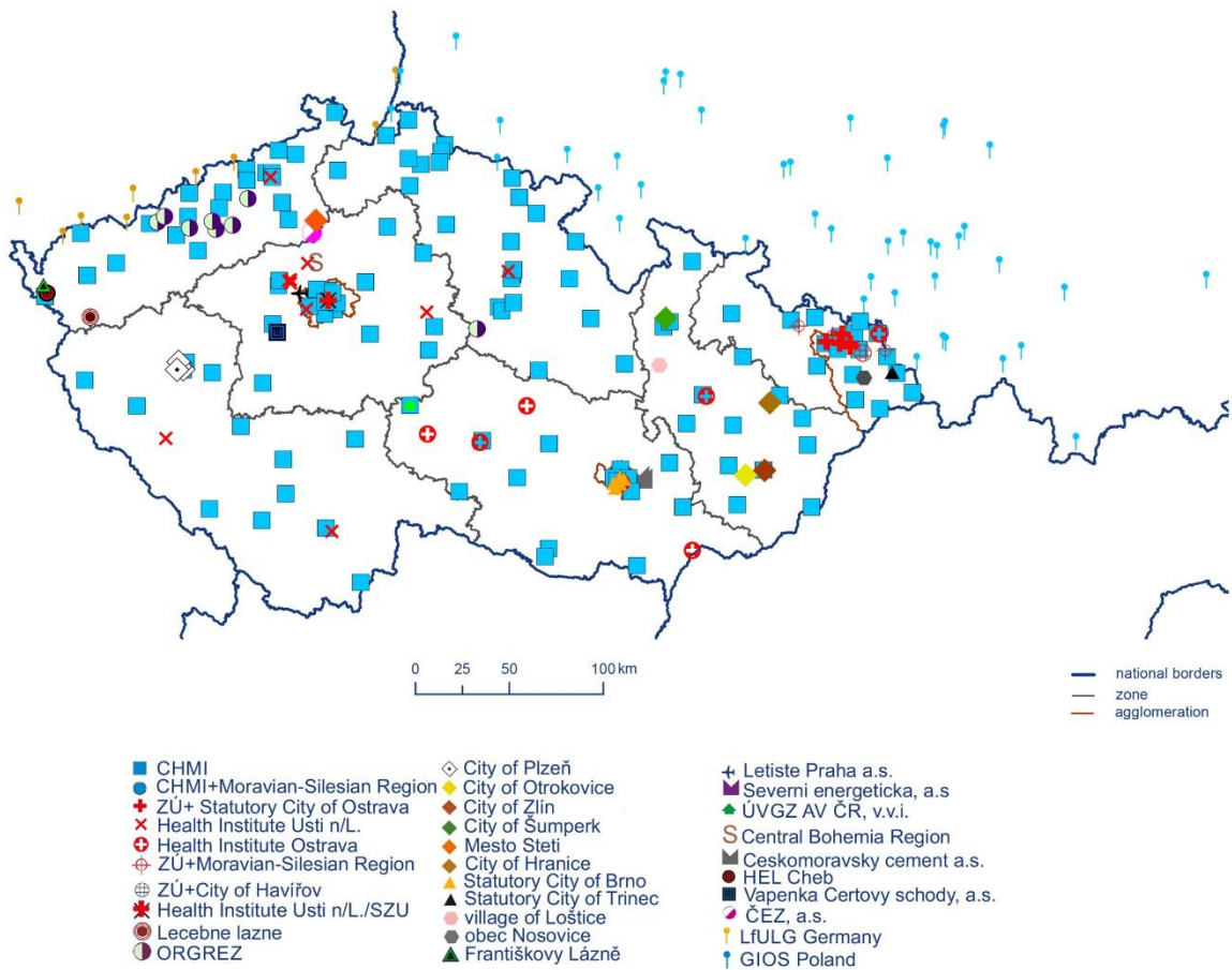
Fig. 3 Major station networks of ambient air quality monitoring, 2020
