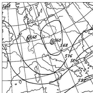
Obr. 14 Mapa hladiny 500 hPa z 6. 7. 1997 12 UTC. Fig. 14. Chart of the 500 hPa level, 6 July 1997, 12 UTC.
