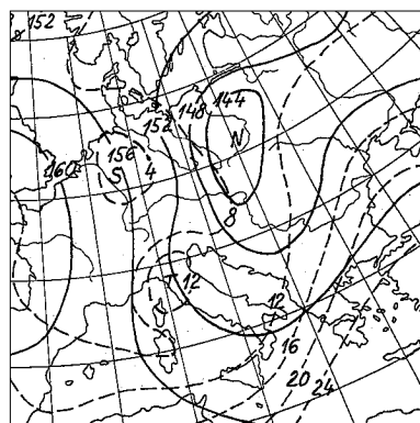
Obr. 13 Mapa hladiny 850 hPa z 6. 7. 1997 12 UTC. Fig. 13. Chart of the 850 hPa level, 6 July 1997, 12 UTC.
