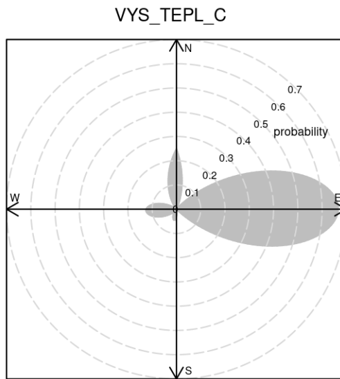
CPF at the 95th percentile (=2.6)
