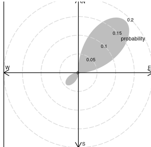
CPF at the 95th percentile (=6.4)
