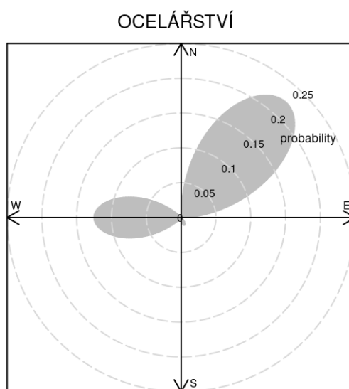
CPF at the 95th percentile (=0.7)
