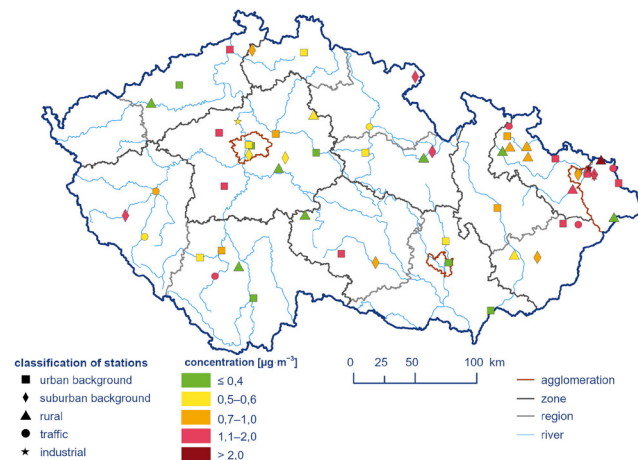
Annual average benzo[a]pyrene concentrations in the Czech Republic, 2024.
