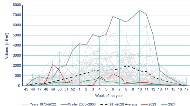
Development of snow storage on the territory of the Czech Republic in individual winter periods since 1970.
