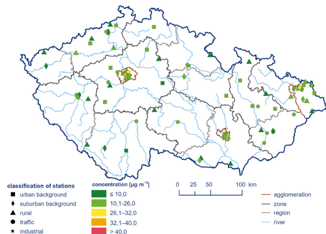
Annual average concentration of \text{NO}_2 at air quality monitoring stations, 2024.
