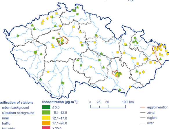
Average annual PM 2.5 concentrations measured at air quality monitoring stations, 2024.
