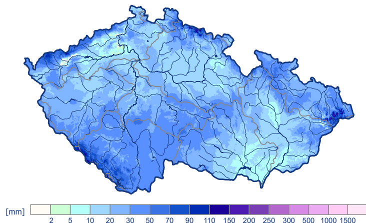
The maximum snow storage water equivalent on the territory of the Czech Republic in winter 2023/2024 (December 4, 2023, 2.122 billion m 3 , runoff 26.9 mm).
