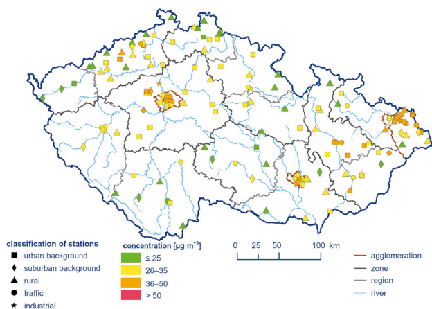
36 th highest 24-hour average concentration of PM 10 measured at air quality monitoring stations, 2024.
