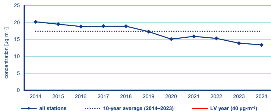
Annual average \text{NO}_2 concentrations (averages for all air quality monitoring stations), 2014–2024.
