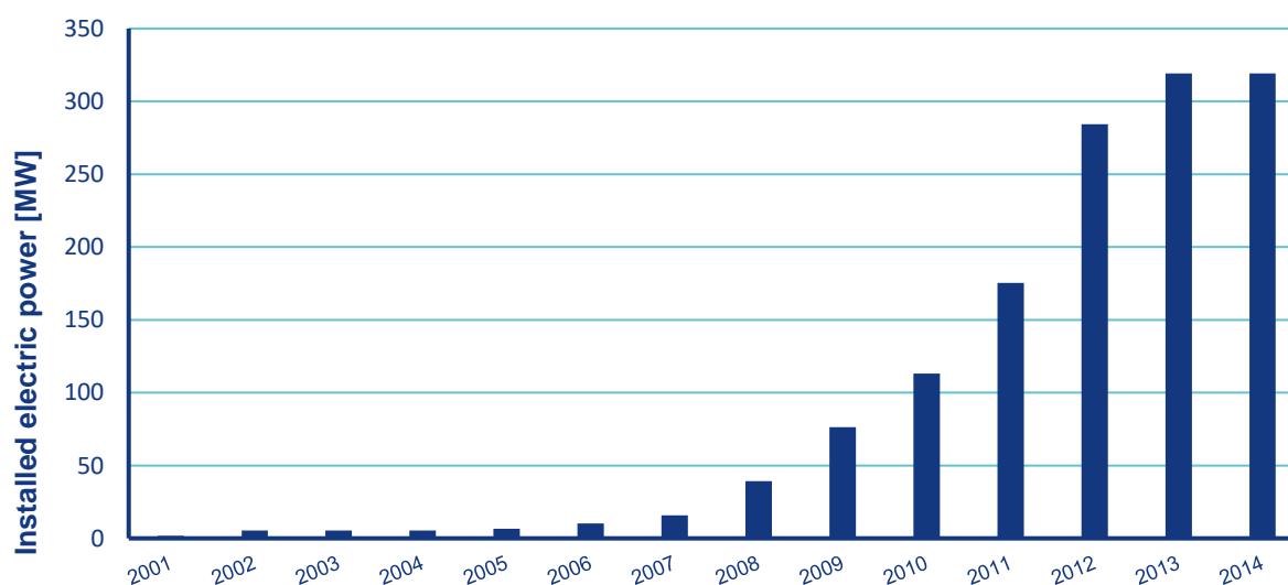
Figure VI.4 Installed electric power of agricultural biogas plants, 2001–2014
