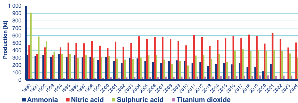
Figure IV.3 Ammonia, sulphuric acid, nitric acid and titanium dioxide production, 1990–2024
