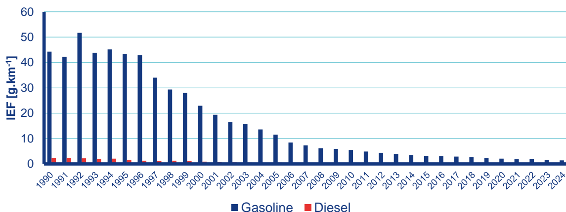
Figure III.13 CO implied emission factors for passenger cars, 1990–2024
