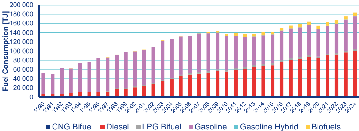
Figure III.12 Annual fuel consumption by passenger cars, 1990–2024
