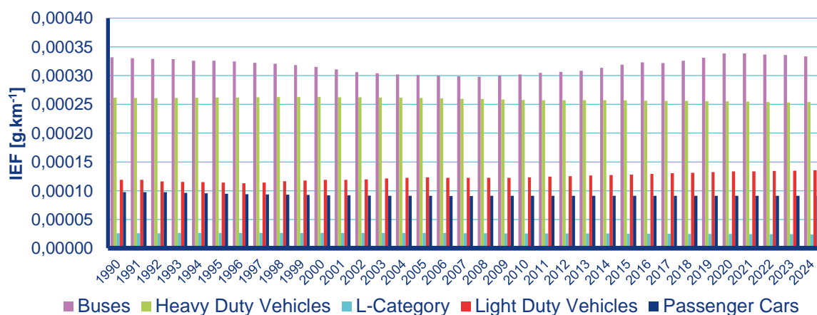
Figure III.21 Pb implied emission factors from tyre, brake and road abrasion, 1990–2024
