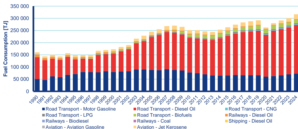
Figure III.6 Annual fuel consumption by all modes of transport, 1990–2024
