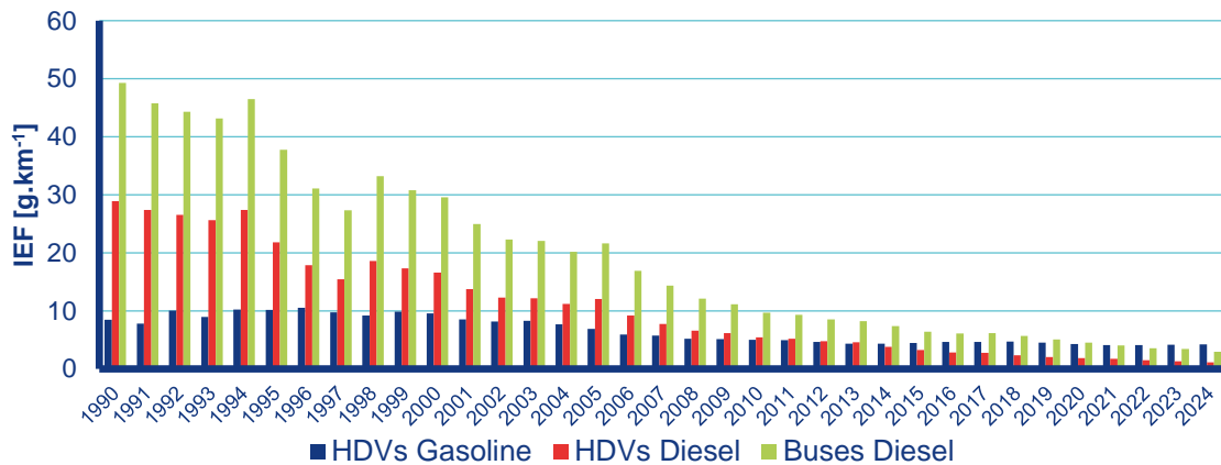
Figure III.16 NO x implied emission factors for heavy-duty vehicles and buses, 1990–2024
