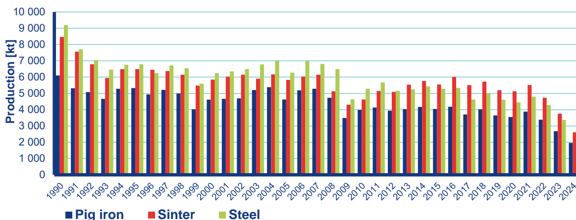
Figure IV.4 Pig iron, steel and sinter production, 1990–2024
