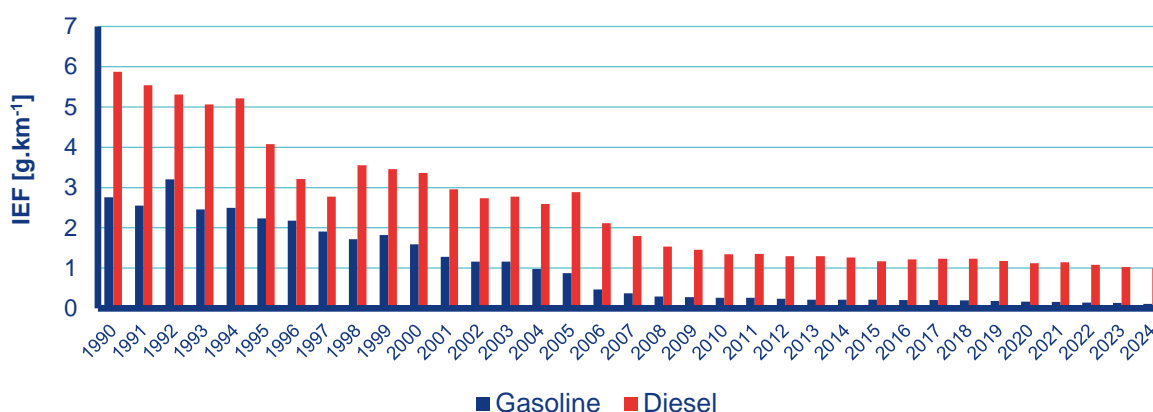
Figure III.15 NO x implied emission factors for light-duty vehicles, 1990–2024
