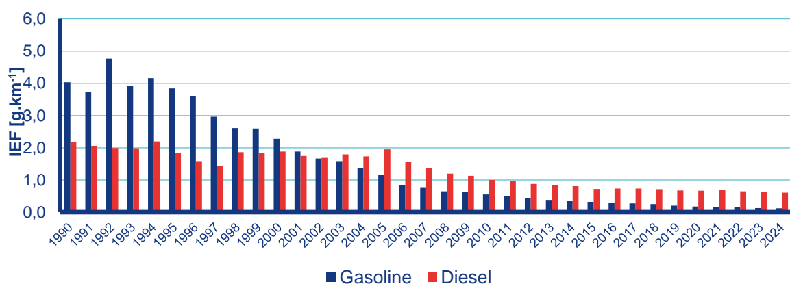
Figure III.14 NO x implied emission factors for passenger cars, 1990–2024
