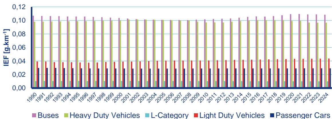
Figure III.20 PM 10 implied emission factors from tyre, brake and road abrasion, 1990–2024
