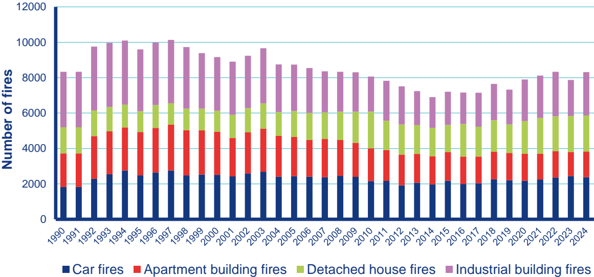
Figure VI.11 Fires, 1991–2024
