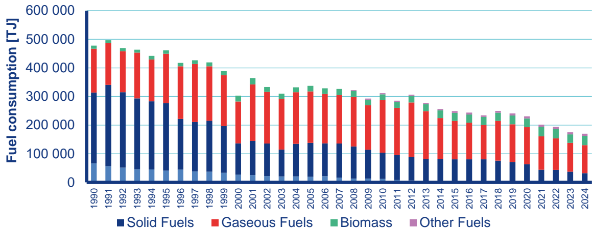
Figure III.2 Fuel consumption for GNFR sector B_Industry, 1990–2024
