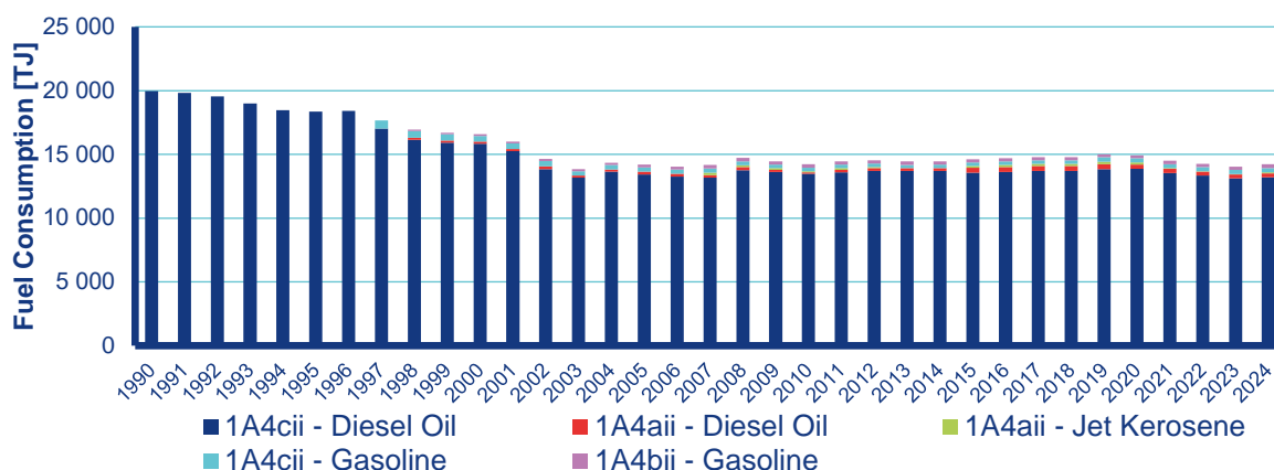
Figure III.22 Annual fuel consumption by non-road mobile machinery, 1990–2024
