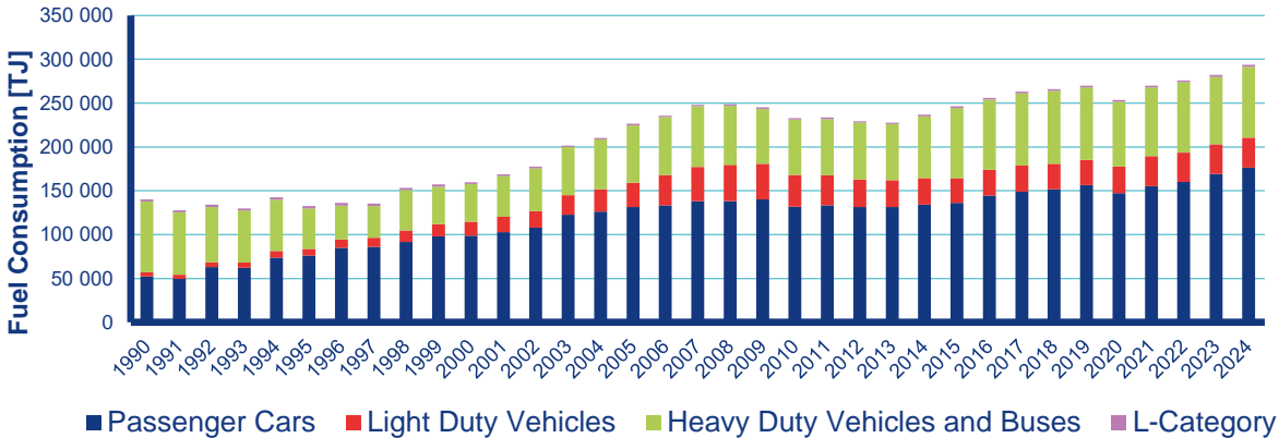
Figure III.7 Annual fuel consumption by road transport, 1990–2024
